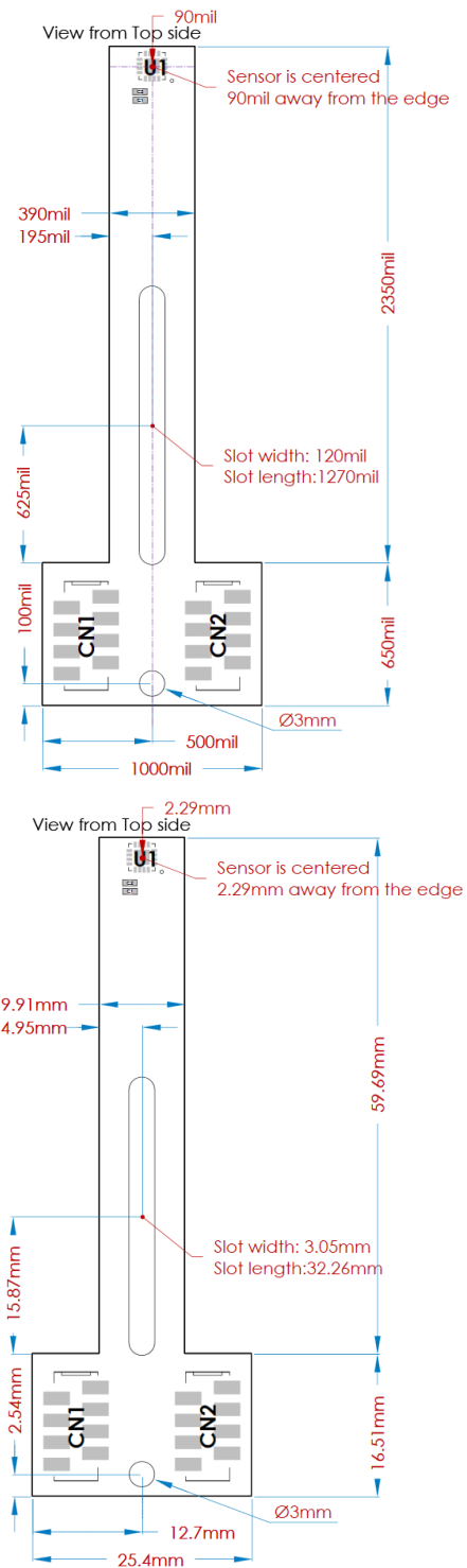
Figure 18: LT Type 2 Mechanical Drawing, mil = 0.001" = 0.0254mm
