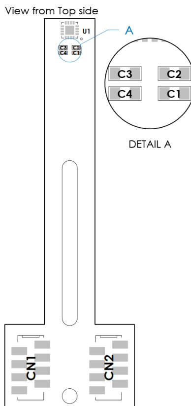
Figure 5: Type 1 Board Assembly View
