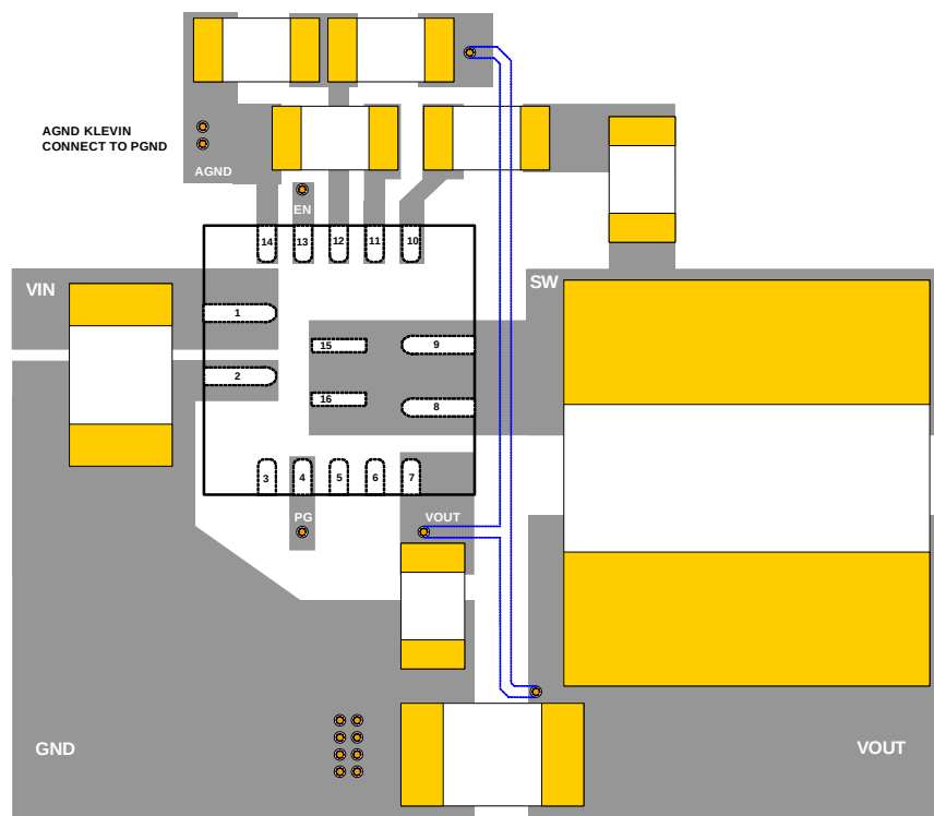
Figure 15: Recommend Layout
