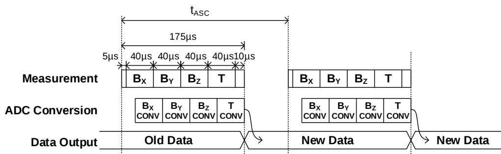
Figure 10: Measuring Sequence in ASC Mode
