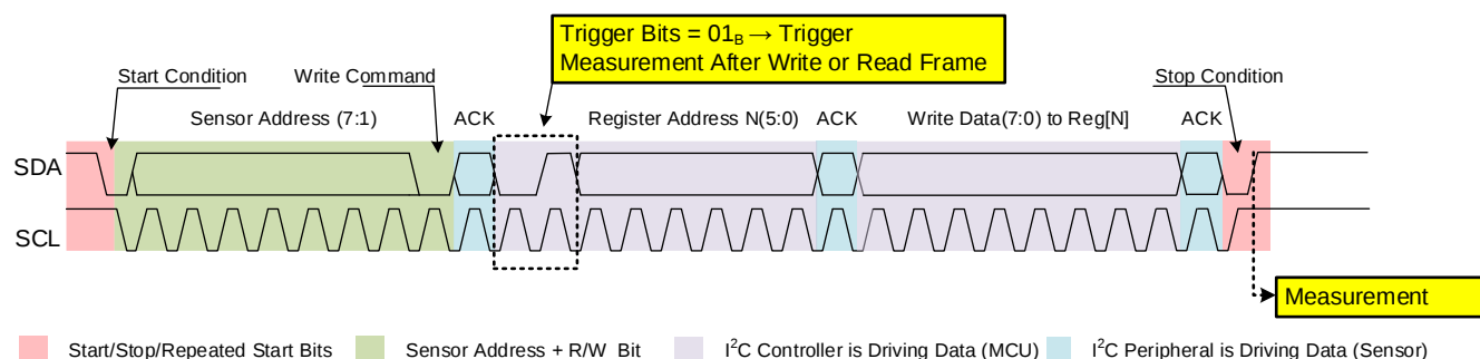
Figure 17: Example of I²C Trigger (Trigger Bits = 01B)
