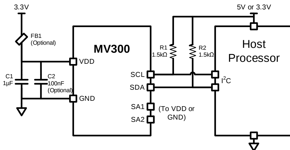
Figure 24: Typical Application Circuit (I 2 C Version)
