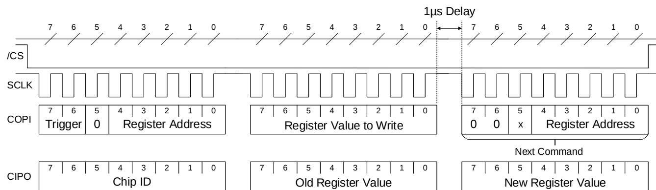
Figure 22: SPI Write Command
