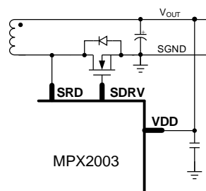
Figure 8: V_{\text{DD}} Supply from the Output
