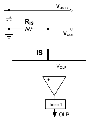
Figure 21: OLP through the IS Pin
