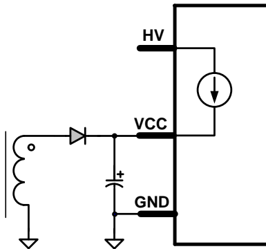
Figure 13: Start-Up Circuit
