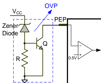
Figure 20: OVP through PEP
