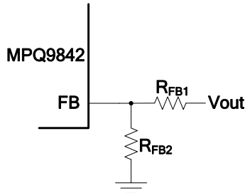
Figure 4: Feedback Network
