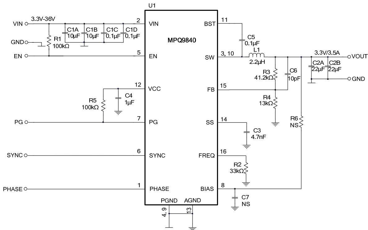
Figure 10: V_{OUT} = 3.3V , F_{sw} = 2.2MHz
