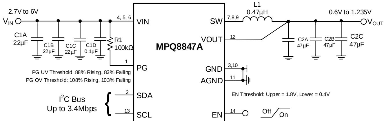
Figure 3: Typical Application Circuit (f SW = 1.25MHz, V OUT = 0.95V)
