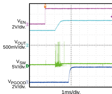
Pre-Bias Start-Up
