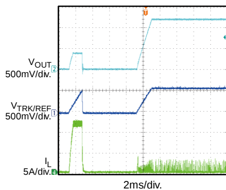
OCP Recovery
