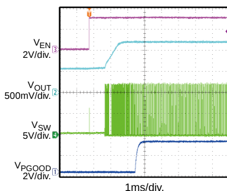
Pre-Bias Start-Up
