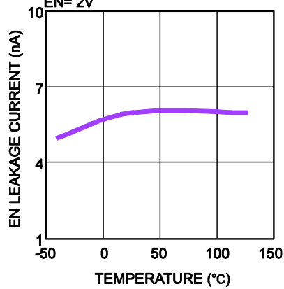
EN Leakage Current vs. Temperature EN= 2V
