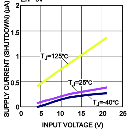
Supply Current (Shutdown) vs. Input Voltage EN= 0V
