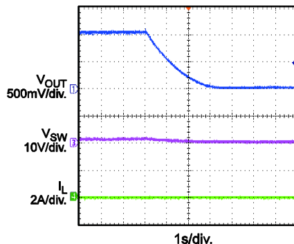
Thermal Shutdown
