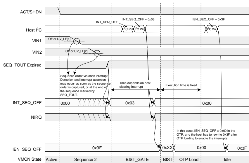
Figure 11: Off Sequence Monitoring (AT_SHDN Enabled)
