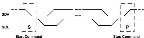
Figure 22: Start and Stop Commands
