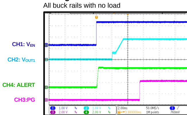
PG and ALERT during Start-Up through EN All buck rails with no load
