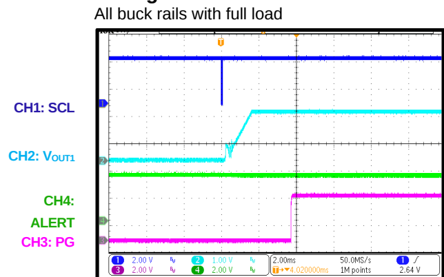
PG and ALERT during Start-Up through PMBus All buck rails with full load
