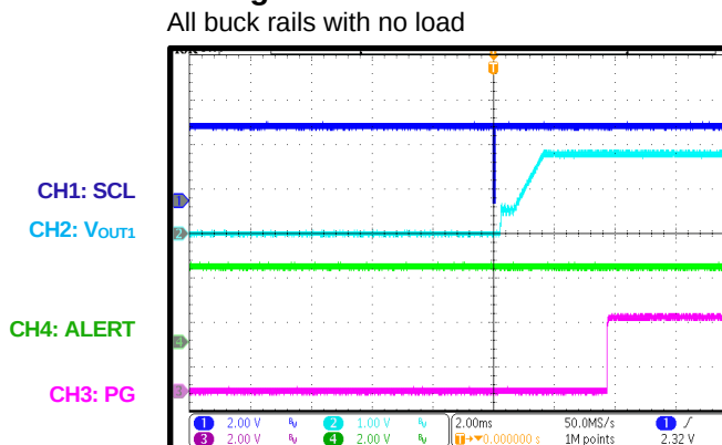
PG and ALERT during Start-Up through PMBus All buck rails with no load
