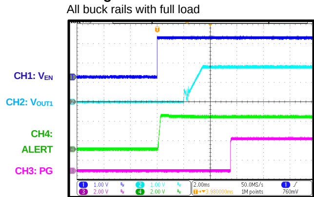
PG and ALERT during Start-Up through EN All buck rails with full load
