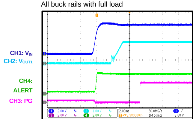
PG and ALERT during Start-Up through VIN All buck rails with full load
