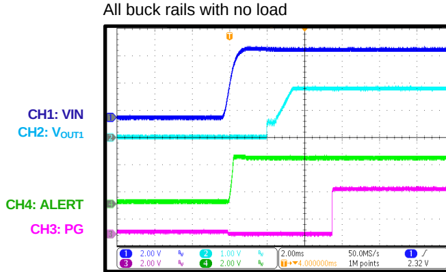
PG and ALERT during Start-Up through VIN All buck rails with no load
