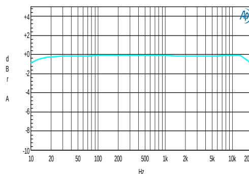
Frequency Response 1W, 4Ω + 33μH
