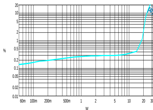
THD + N vs. P_{OUT} 4Ω + 33μH
