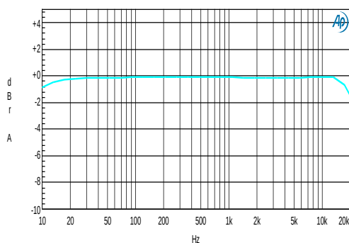
Frequency Response 1W, 8Ω + 66μH
