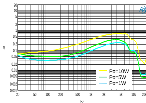
THD + N vs. Frequency 8Ω + 66μH
