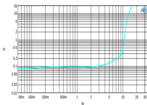
THD + N vs. P_{OUT} 8Ω + 66μH
