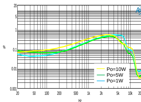
THD + N vs. Frequency 4Ω + 33μH
