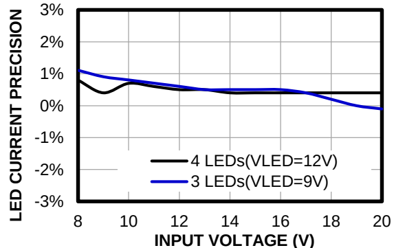
I_{LED} Precision vs. Input Voltage
