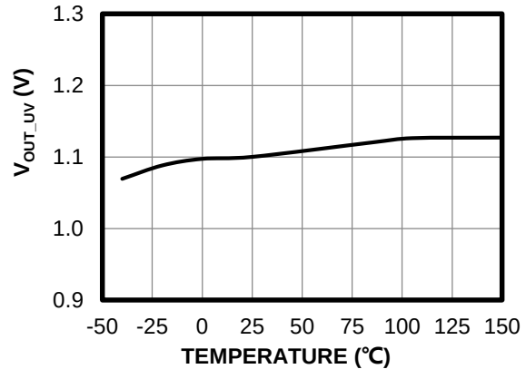
V_{OUT\_UV} Threshold vs. Temperature Buck mode
