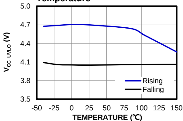
VCC UVLO Threshold vs. Temperature
