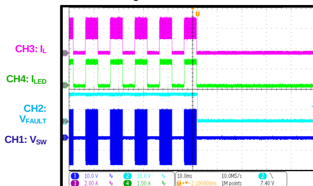
ISET Open Fault after IC Starts Up PWM dimming
