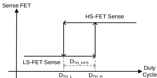
Figure 4: Current-Sense MOSFET vs. Duty Cycle
