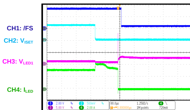
ISET Pin Short Protection
