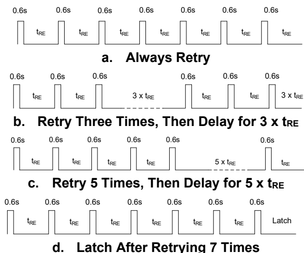
Figure 7: Rotor Deadlock Protection and Retry Time
