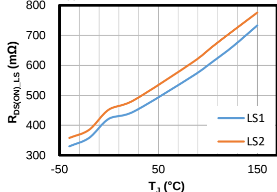
LS-FET On Resistance vs. Junction Temperature
