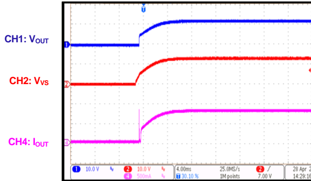
V_{VS} Start-Up HS on, I_{OUT} = 800mA
