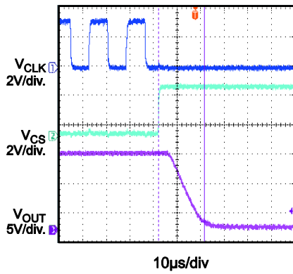
Output Delay Time LS ON
