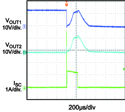
SCP SCT=0, OUT1 short to OUT2
