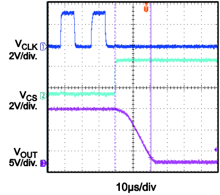
Output Delay Time HS OFF
