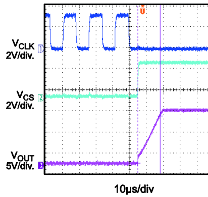
Output Delay Time LS OFF
