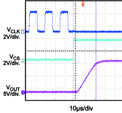
Output Delay Time HS ON
