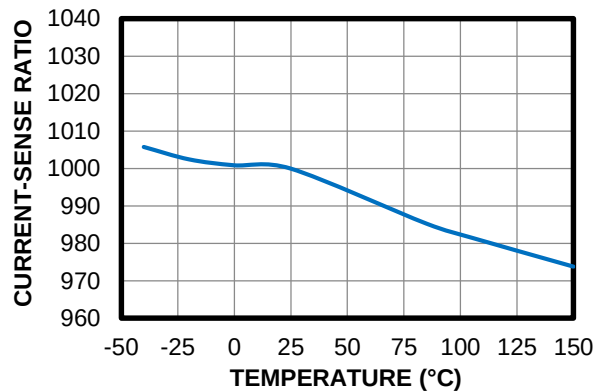
Current-Sense Ratio vs. Temperature
