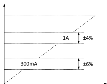
Figure 3: Current-Sense Accuracy
