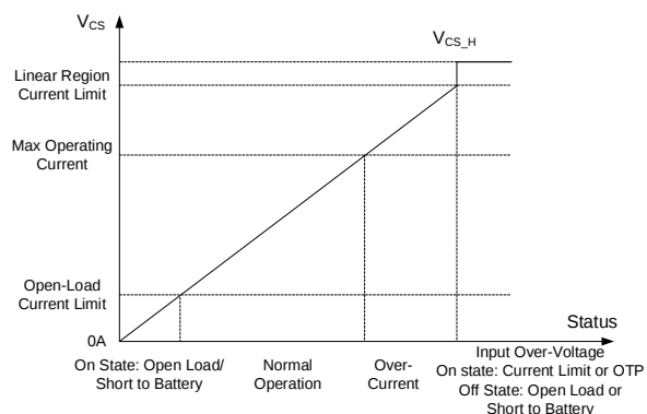
Figure 4: V_{CS} Range and IC Status
