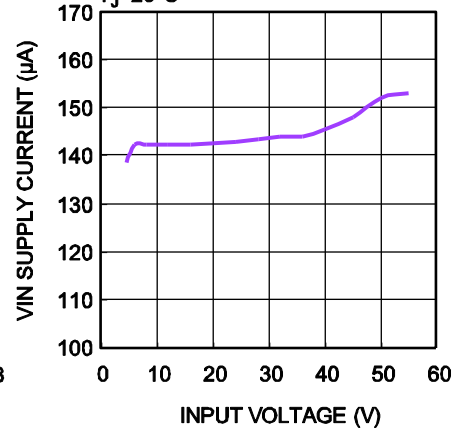
V_{IN} Quiescent Current vs. Input Voltage
