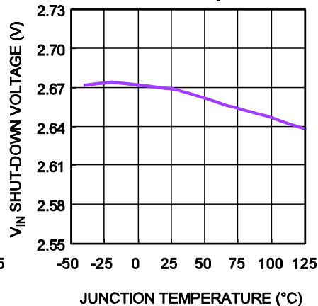
V_{IN} Shut-down vs. Junction Temperature
