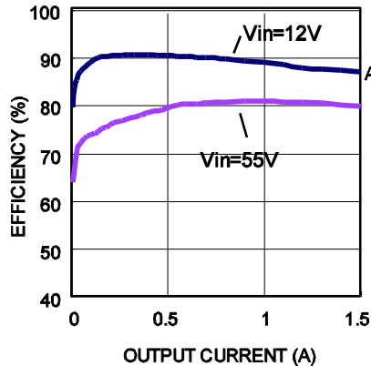
Efficiency @ V_{OUT}=5V
