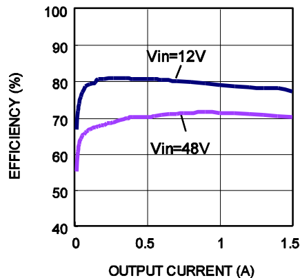
Efficiency @ V_{OUT}=2.5V
