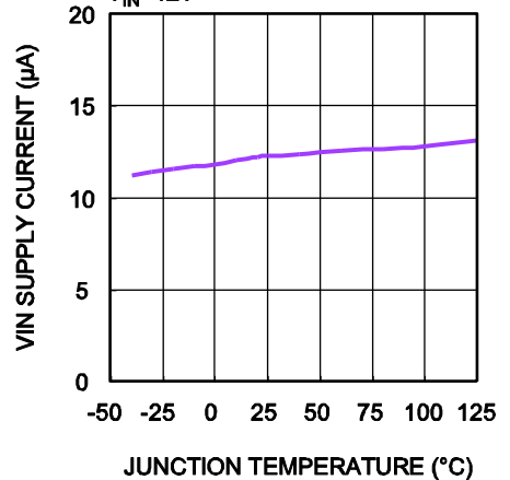
Shutdown Current vs. Junction Temperature
