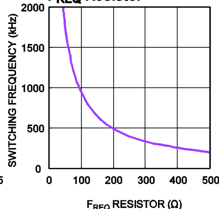
Frequency vs. F_{REQ} Resistor
