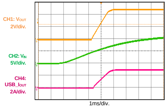
Power Start-Up
