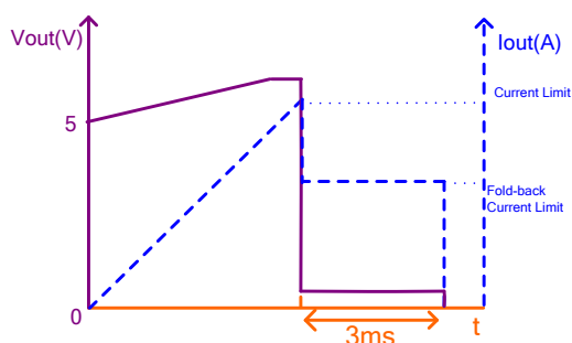
Figure 4: Over-Current Limit
