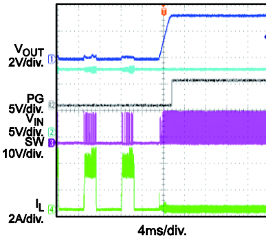
SCP Recovery I_{OUT} = 0A
