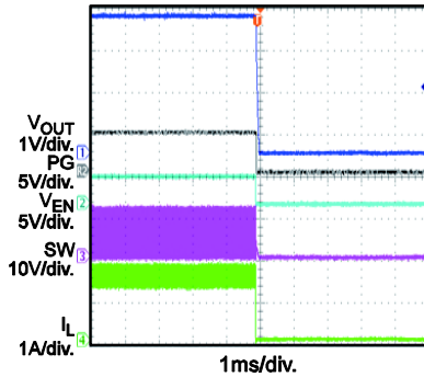
Shutdown through Enable I_{OUT} = 1.5A
