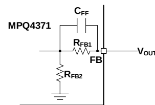
Figure 13: Feedback Divider Network of Fixed-Output Version
