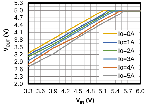
Low Dropout
