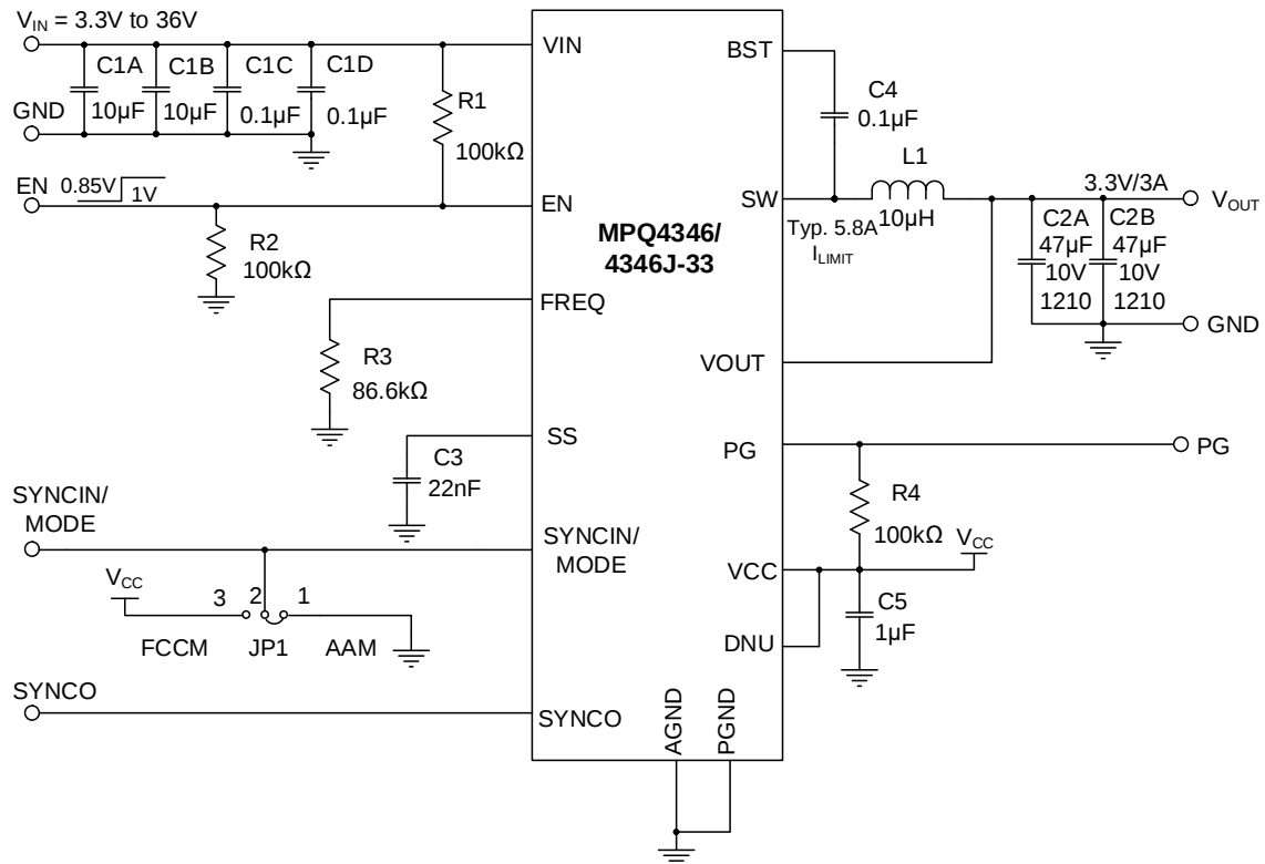
Figure 12: Typical Application Circuit ( V_{OUT} = 3.3V , f_{SW} = 410kHz )
