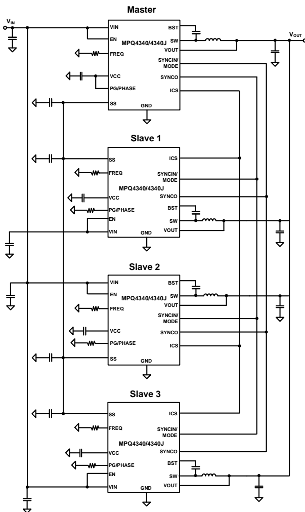
Figure 5: 4-Phase Configuration
