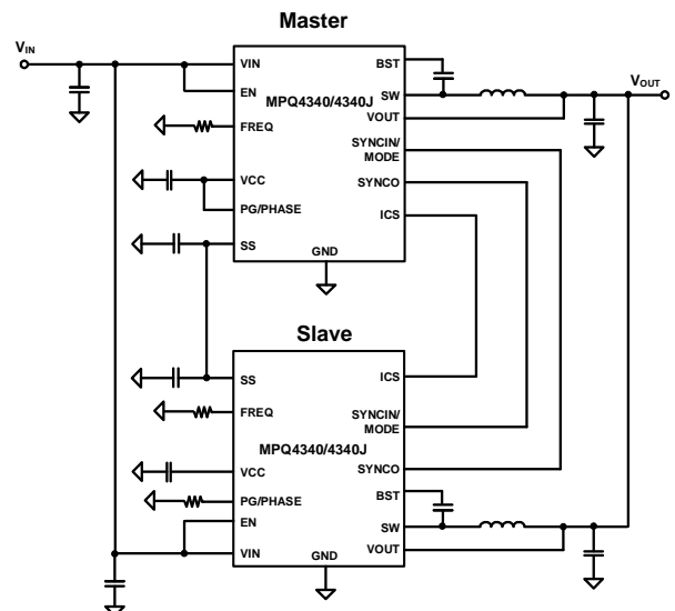
Figure 4: 2-Phase Configuration
