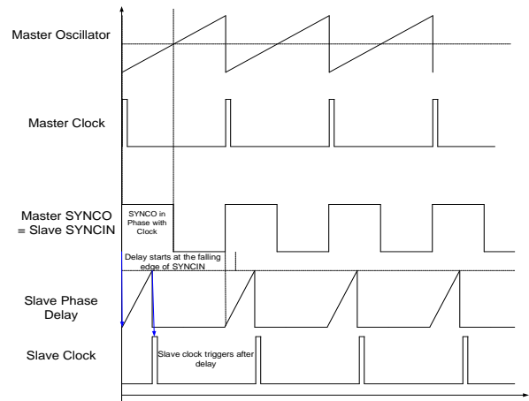
Figure 3: SYNCIN and SYNCO Scheme
