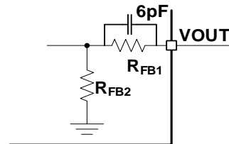
Figure 10: Feedback Divider Network for Fixed-Output Version
