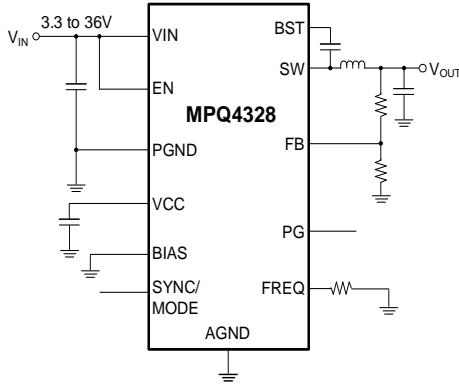
Figure 1: Typical Application (Adjustable Output)
