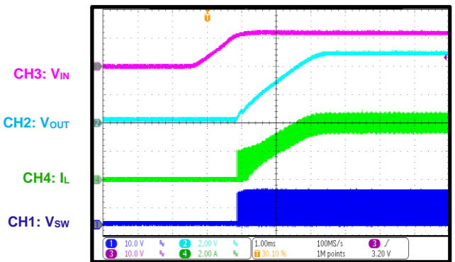
Start-Up through VIN V_{IN} = 12A , I_{OUT} = 4A
