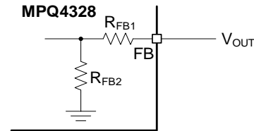
Figure 9: Feedback Divider Network for Fixed-Output Version
