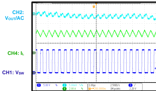
Steady State V_{IN} = 12V , I_{OUT} = 4A
