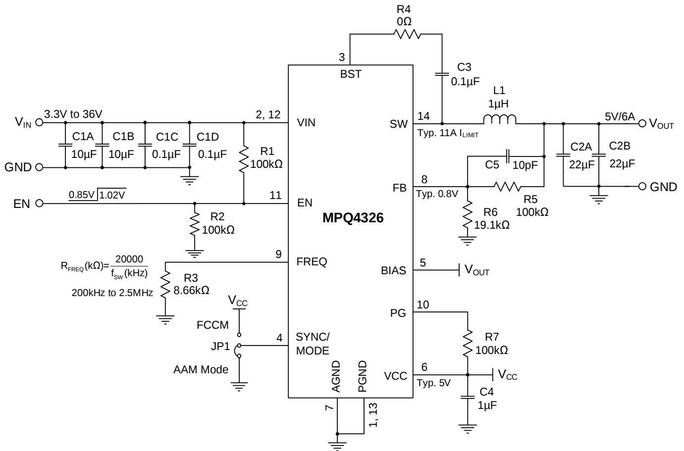
Figure 7: Typical Application Circuit (V OUT = 5V, f sw = 2.2MHz)
