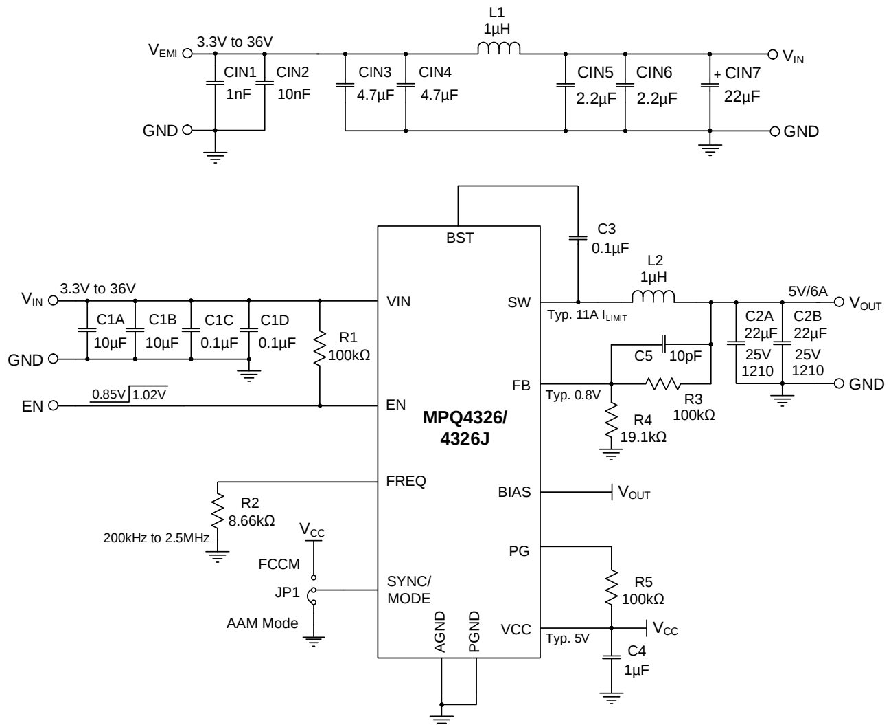
Figure 17: Typical Application Circuit ( V_{\text{OUT}} = 5\text{V} , f_{\text{sw}} = 2.2\text{MHz} with EMI Filters)
