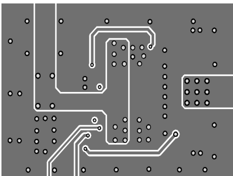
Mid-Layer 2
