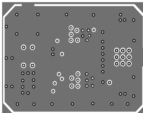
Mid-Layer 1
