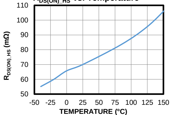
R_{DS(ON)_HS} vs. Temperature
