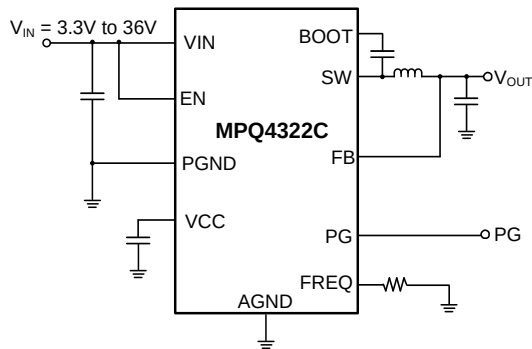
Figure 2: Typical Application Circuit (Fixed Output)
