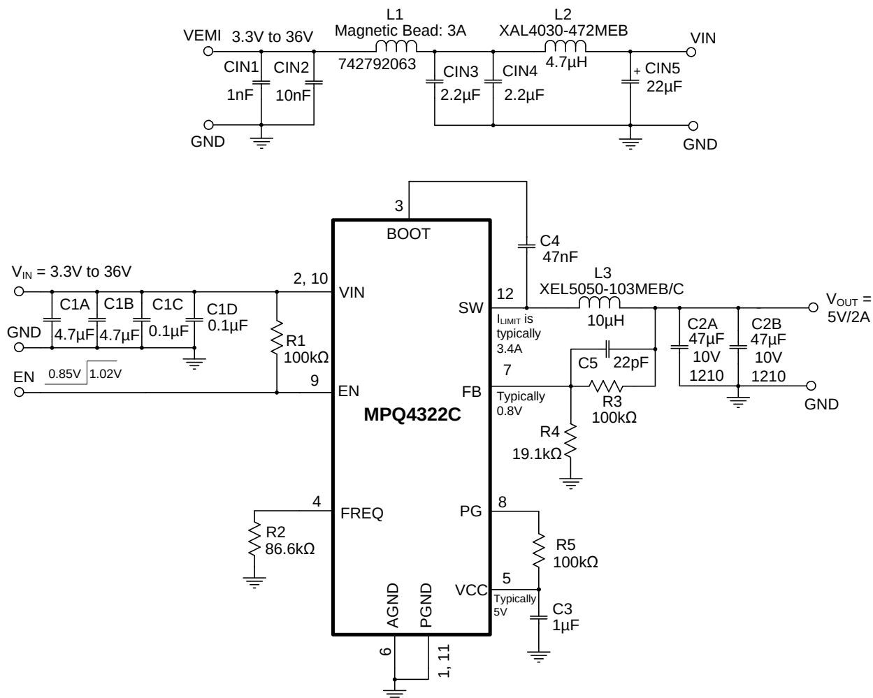
Figure 18: Typical Application Circuit (QFN-12, V_{OUT} = 5V , f_{sw} = 415kHz with EMI Filters)
