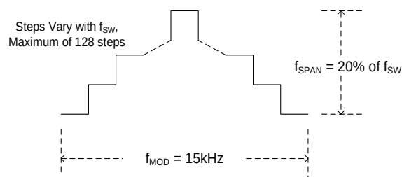
Figure 5: Frequency Spread Spectrum
