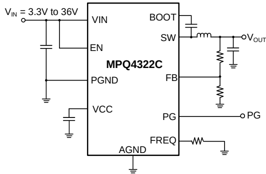
Figure 1: Typical Application Circuit (Adjustable Output)
