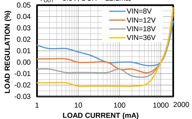
Load Regulation
