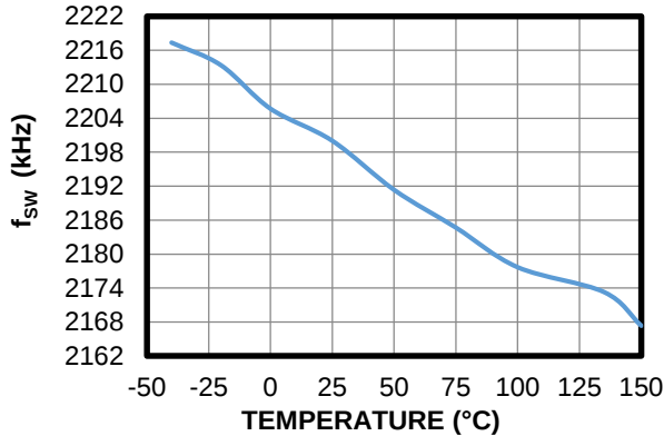
f_{SW} vs. Temperature R_{FREQ} = 15k\Omega
