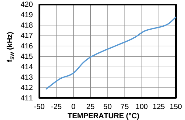
f_{SW} vs. Temperature R_{FREQ} = 86.6k\Omega
