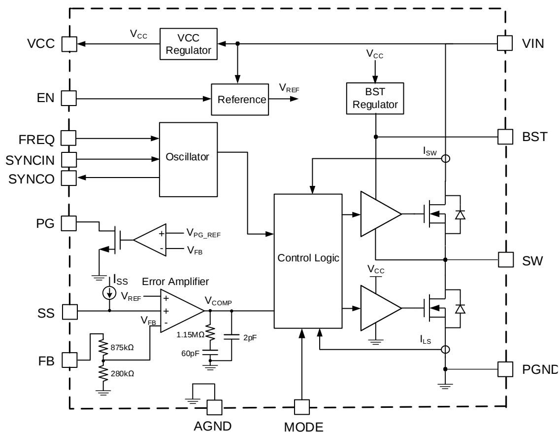
Figure 4: Functional Block Diagram (3.3V Fixed-Output Version)
