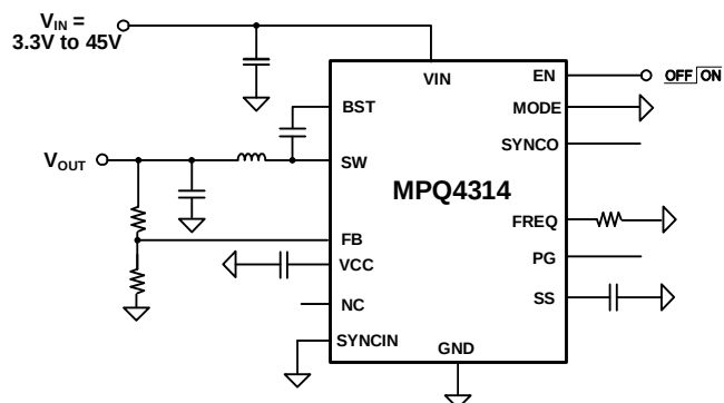
Figure 1: Adjustable-Output Version
