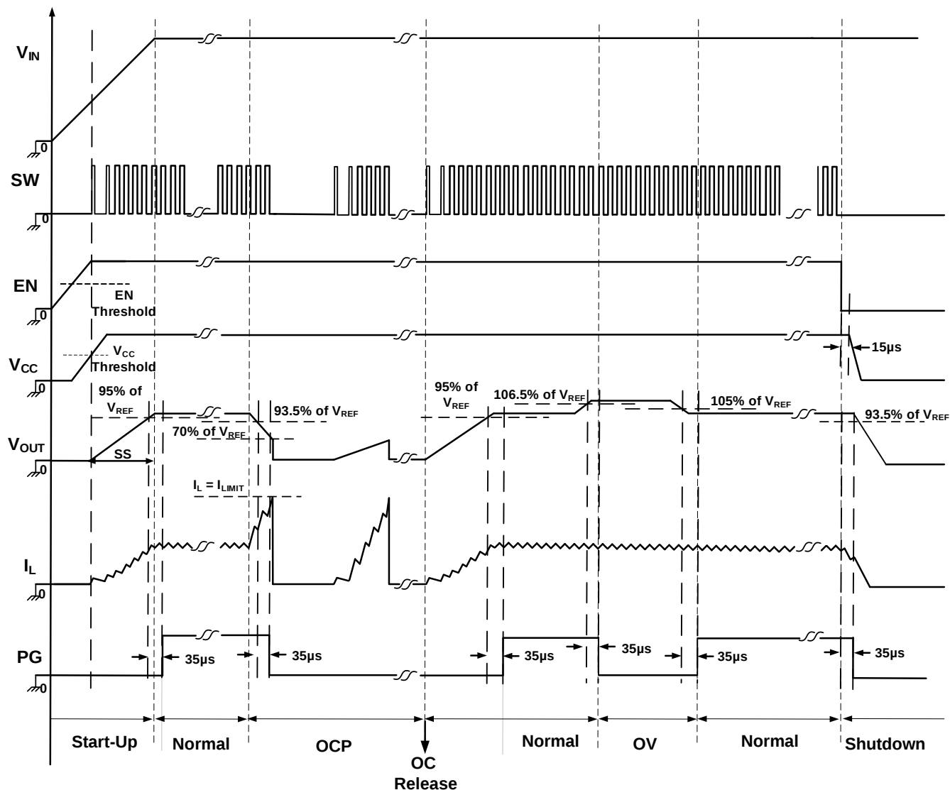
Figure 5: Timing Sequence
