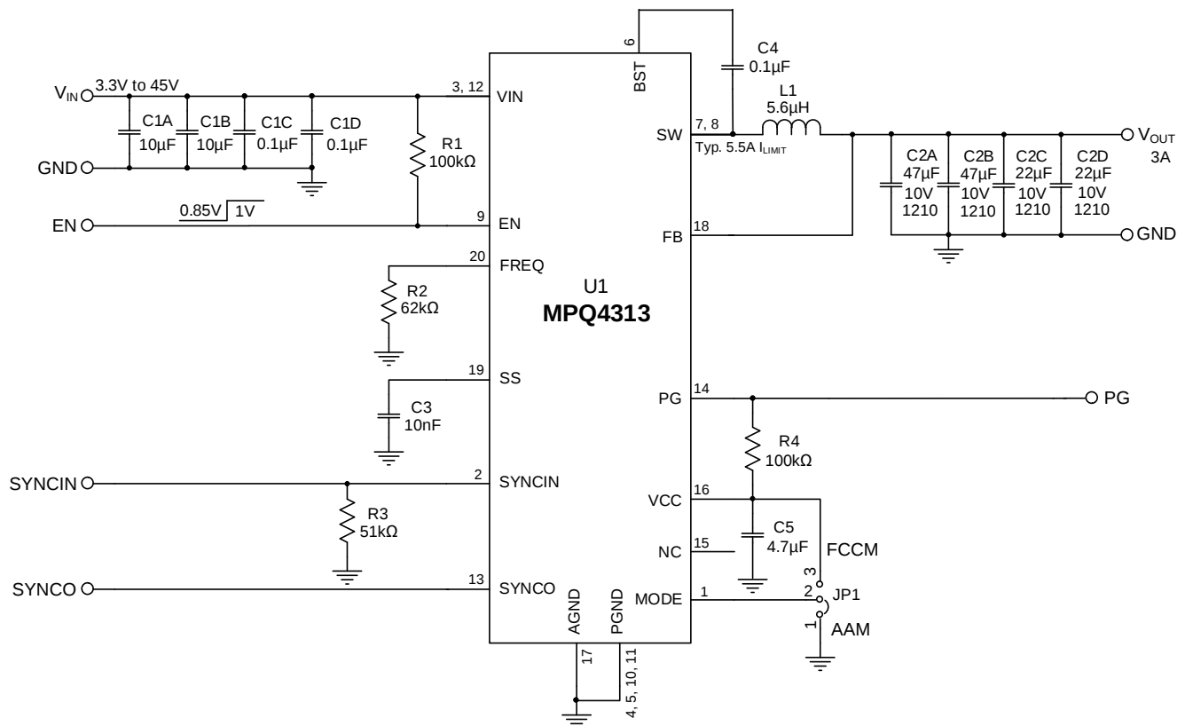
Figure 14: Typical Application Circuit ( f_{SW} = 470kHz , Fixed Output)
