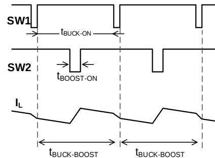
Figure 5: Buck-Boost Waveform
