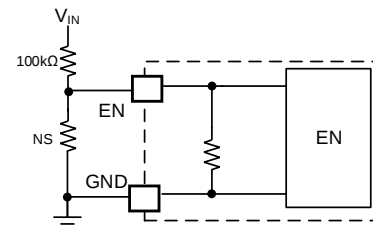
Figure 6: EN Connection
