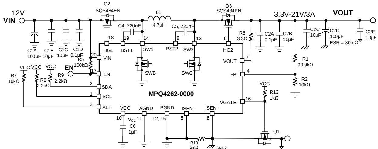
Figure 14: V_{IN} = 12V , V_{OUT} = 3.3V to 21V/3A (OPERATION Set to On) (9)
