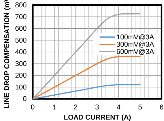
Line Drop Compensation vs. Load Current
