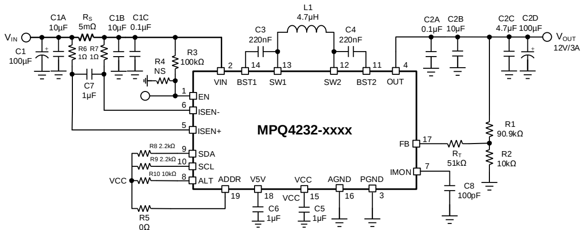
Figure 15: Typical Application Circuit ( V_{IN} = 9V to 16V , V_{OUT} = 12V/3A application with R_S on the input side)
