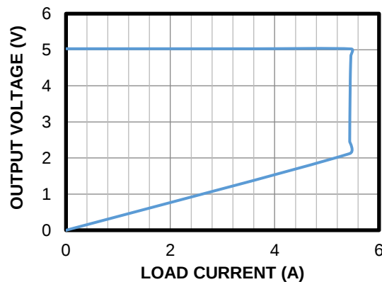
CC/CV Curve
