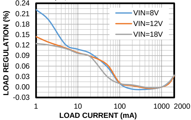
Load Regulation
