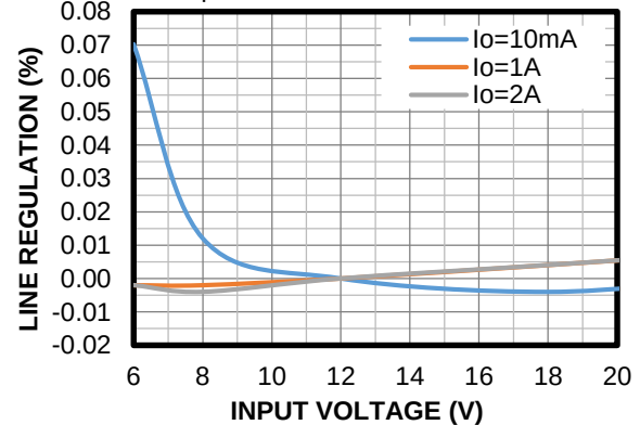
Line Regulation
