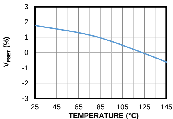
V_{FSET} vs Temperature
