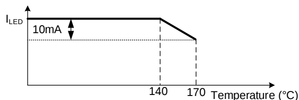
Figure 6: ILED Decrease with Temperature
