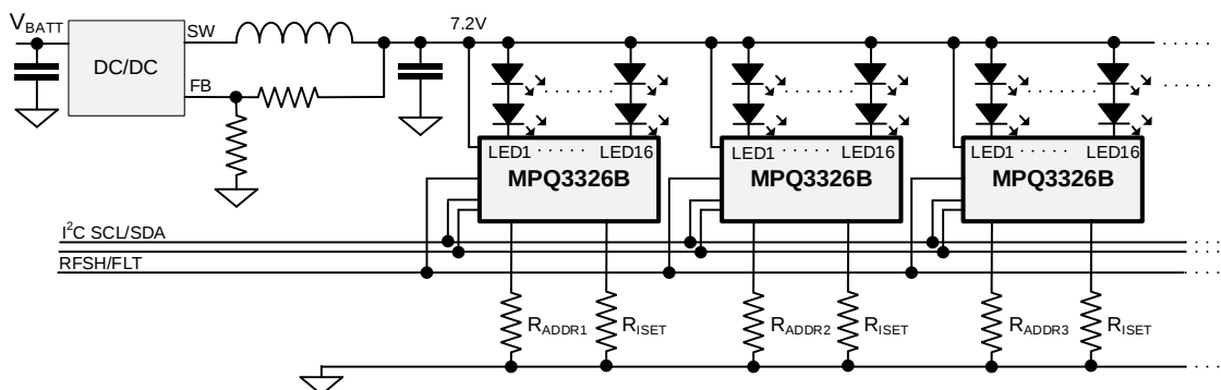
Figure 2: System Application with 2 LEDs in Series
