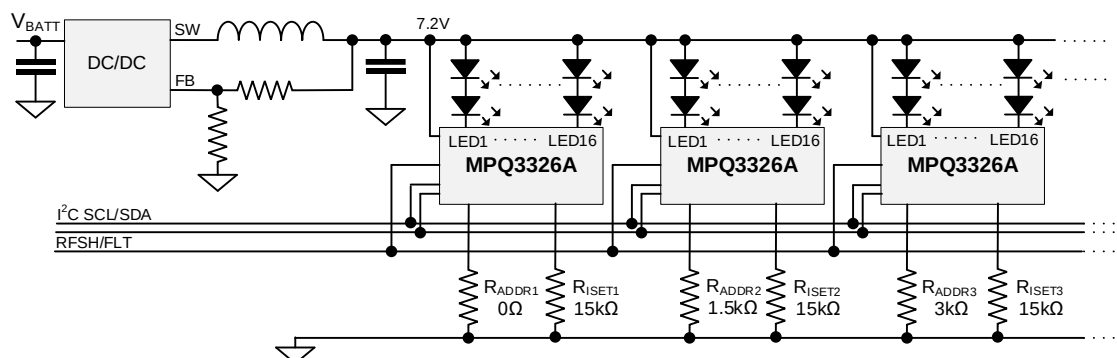
Figure 10: Typical System Application Circuit (2 LED in Series, I_{LED} = 80mA/Channel )
