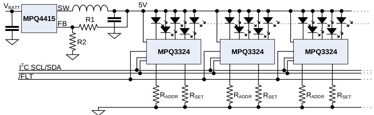
Figure 8: Typical System Application Circuit
