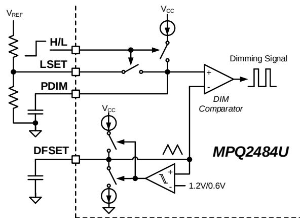
Figure 10: Two-Step Dimming
