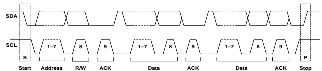
Figure 8: A Complete Data Transfer
