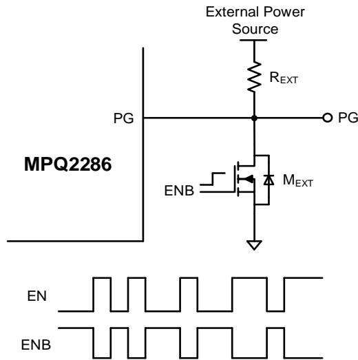
Figure 4: Recommended External Circuit for PG
