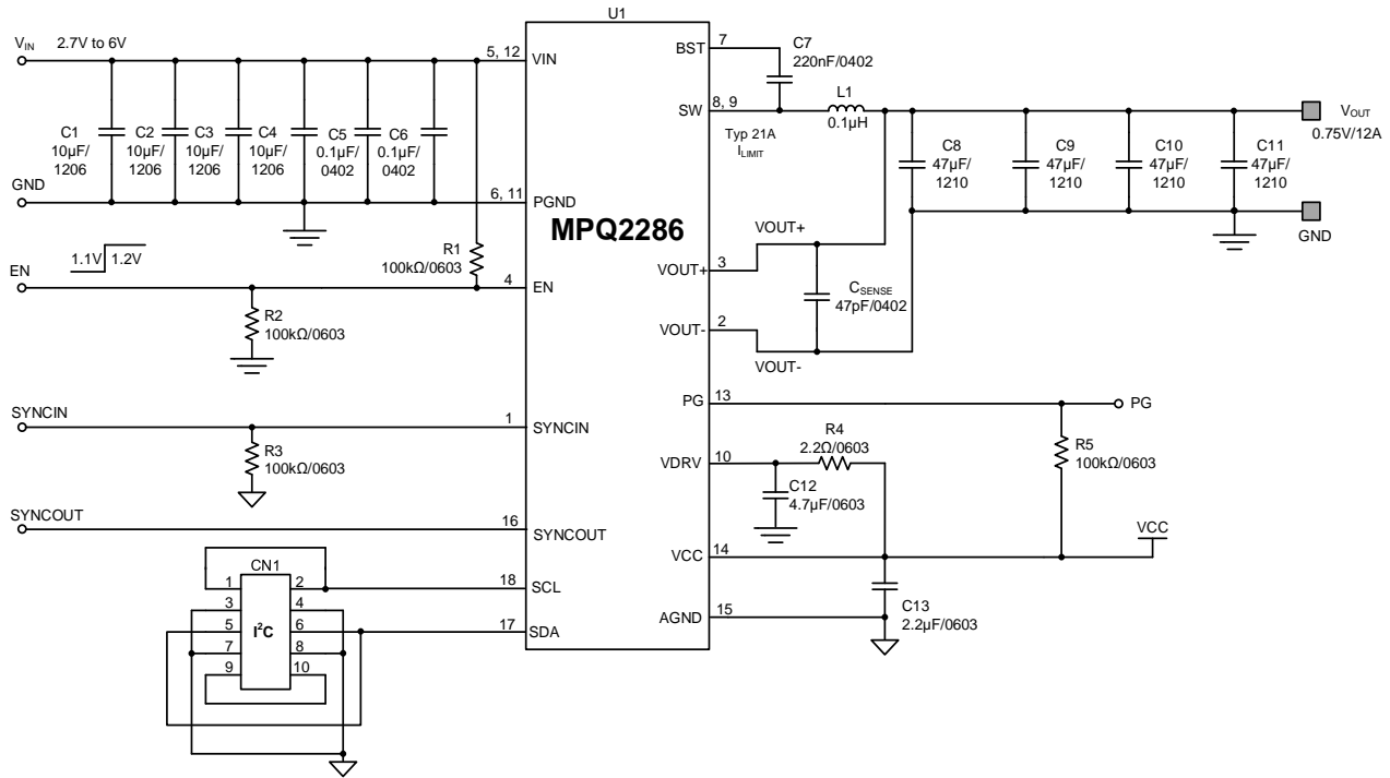
Figure 12: Typical Application Circuit ( V_{OUT} = 0.75V , f_{sw} = 3MHz )
