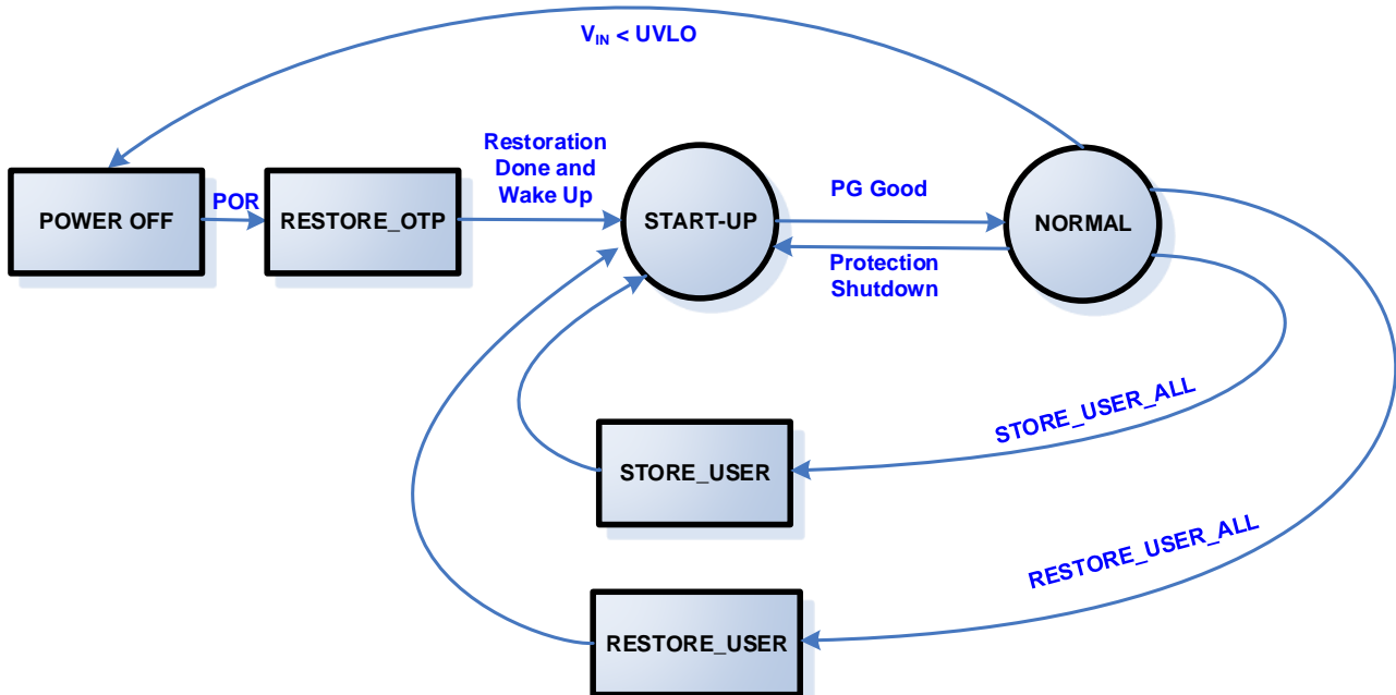
Figure 11: System State Machine
