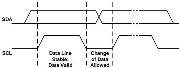
Figure 6: Bit Transfer on the Digital Interface
