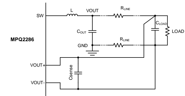
Figure 5: Remote Output Voltage Sensing Circuit
