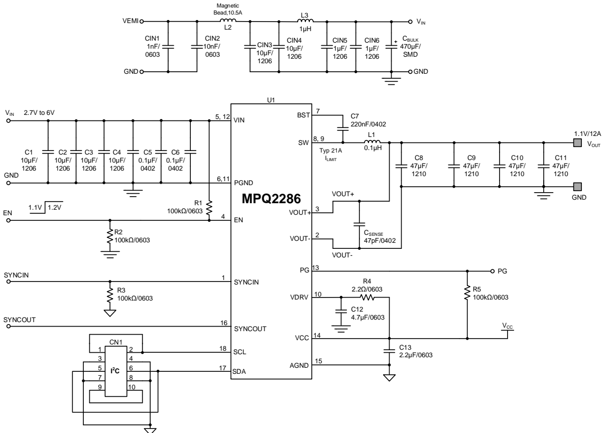
Figure 15: Typical Application Circuit ( V_{OUT} = 1.1V , I_{OUT} = 12A , f_{sw} = 4MHz with EMI Filter)
