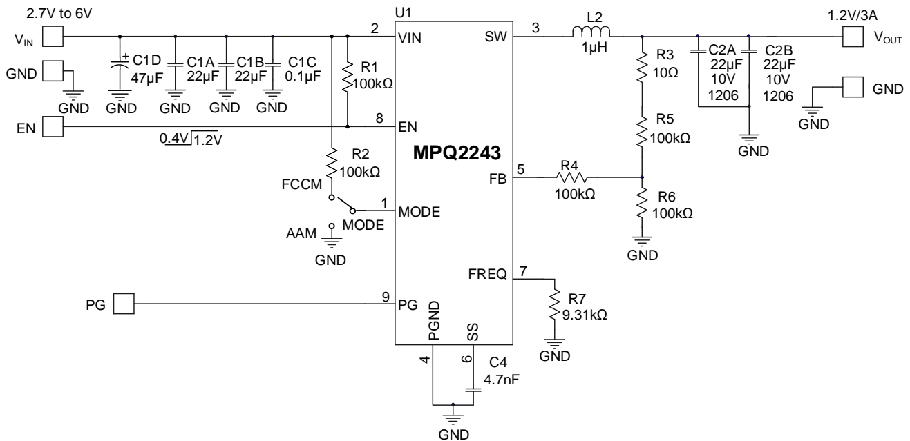
Figure 6: Typical Application Circuit ( V_{OUT} = 1.2V , I_{OUT} = 3A )
