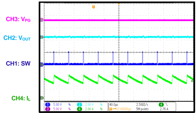
Short-Circuit Protection
