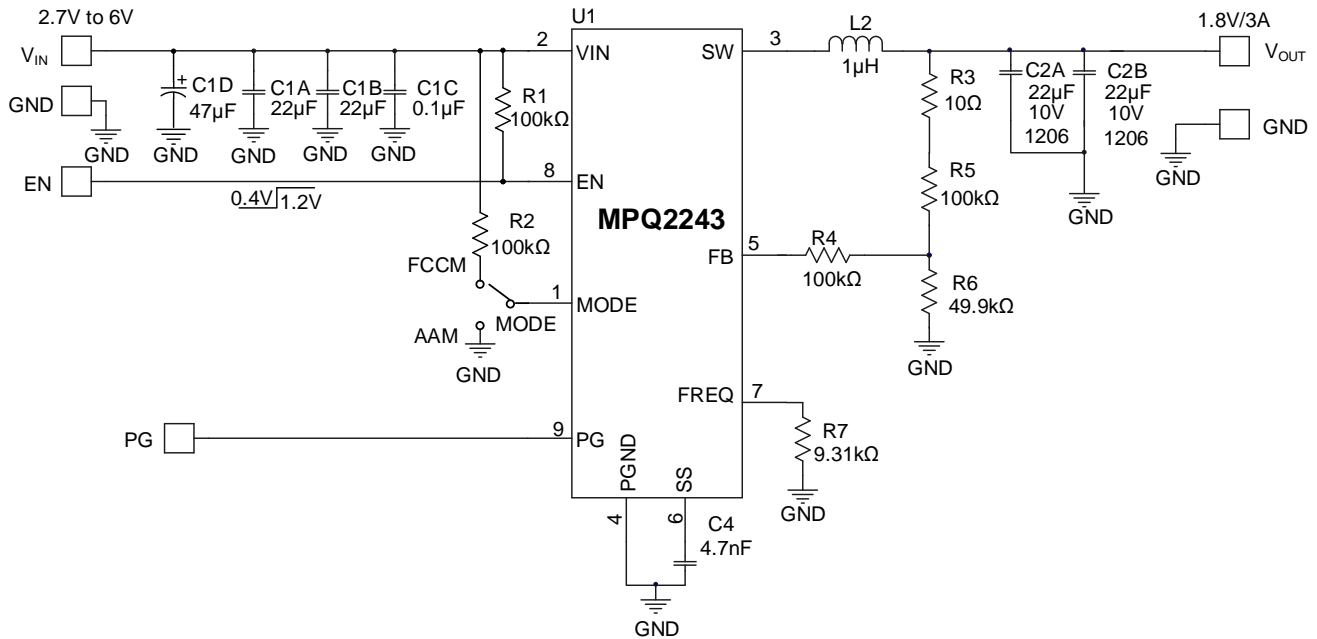
Figure 5: Typical Application Circuit ( V_{OUT} = 1.8V , I_{OUT} = 3A )
