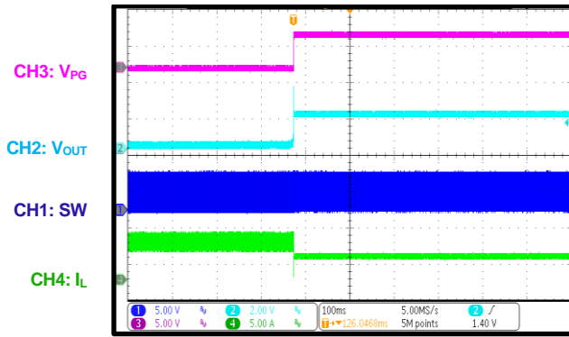
SCP Recovery I_{OUT} = 3A
