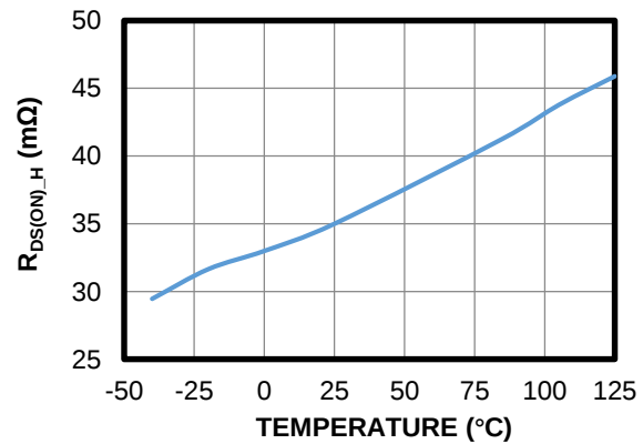
HS-FET On Resistance vs. Temperature (9)
