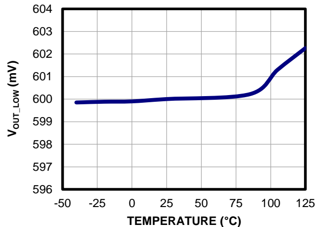
V_{OUT\_LOW} vs Temperature V_{IN} = 5V
